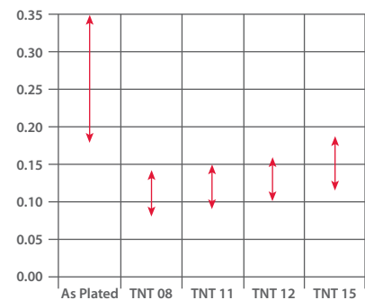
MacDermid Friction Control on Zinc-Nickel Electroplate
